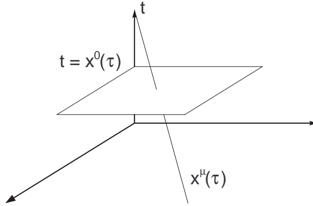
Fig. 4.1 - The space-time trajectory of a point-like particle
