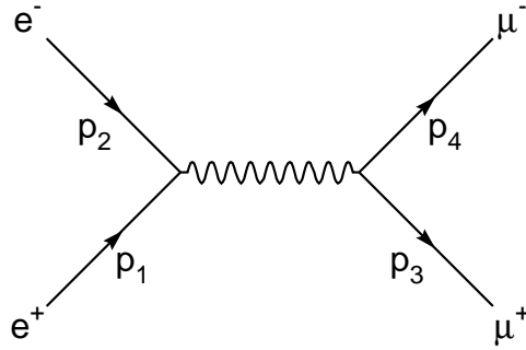
Fig. 9.1 - The Feynman diagram for the scattering e^+e^- \rightarrow \mu^+\mu^- .
