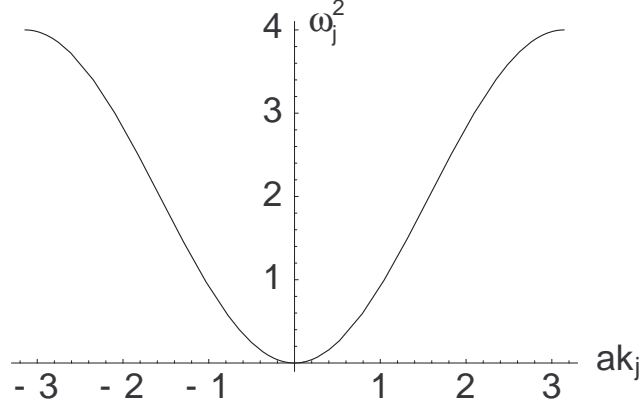
Fig. 1.2 - The first Brillouin zone.
