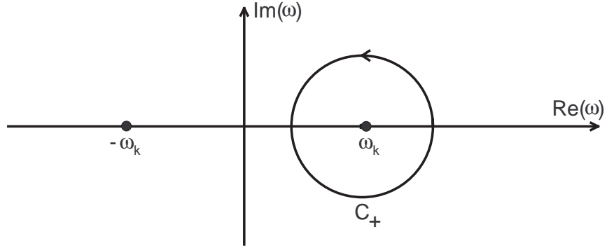
Fig. 7.2 - The integration path C_+ .
