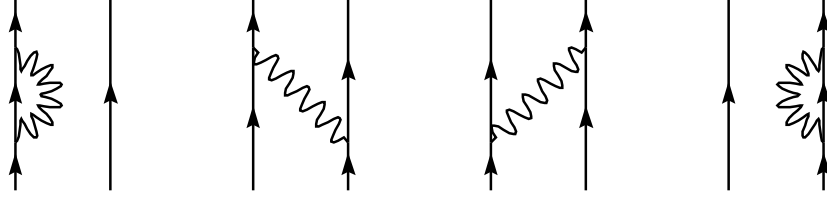
Fig. 7.8 - The graphical description of eq. (7.46).
