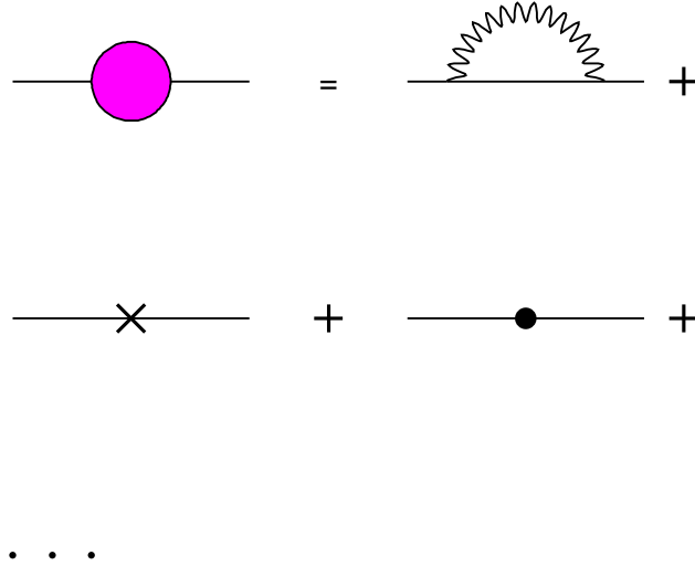
Fig. 10.5 - The counter terms for the self-energy ( p in the figure should be read as \hat{p} ).
