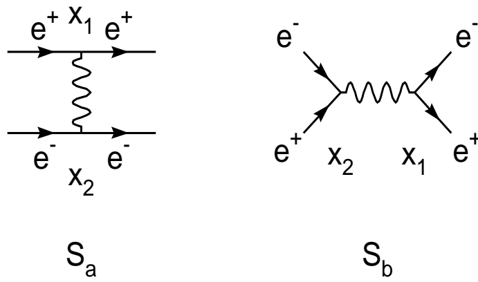
Fig. 8.10 -Inequivalent diagrams for the process e^+e^- \rightarrow e^+e^- .
