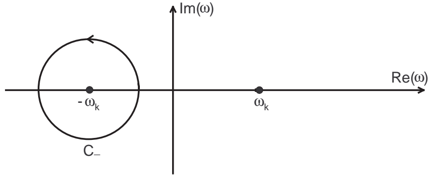
Fig. 7.3 - The integration path C_- .
