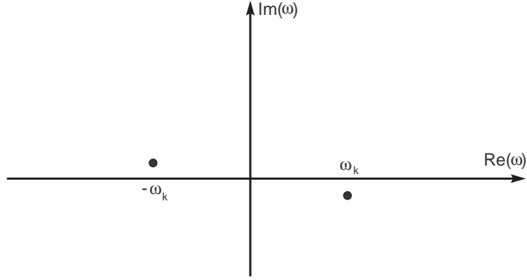
Fig. 7.5 - The position of the poles in the definition of \Delta_F(x) .
