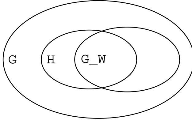
Fig. 6.1 - This figure shows the various groups, G , the global symmetry of the lagrangian, H \in G , the symmetry of the vacuum, and G_W , the group of local symmetries. The broken generators in G_W correspond to massive vector bosons. The broken generators do not belonging to G_W correspond to massless Goldstone bosons. The unbroken generators in G_W correspond to massless vector bosons.
