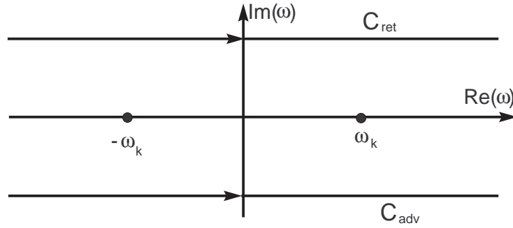
Fig. 7.7 - The integration paths for G_{\text{ret}} and G_{\text{adv}} .
