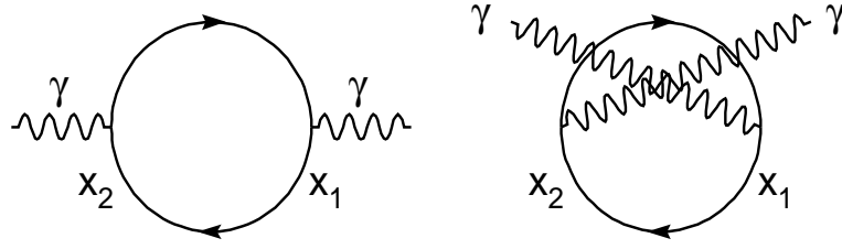
Fig. 8.12 -Photon self-energy.
