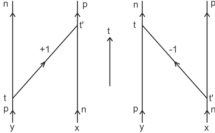
Fig. 7.1 - The two probability amplitudes contributing to the process np \rightarrow np .
