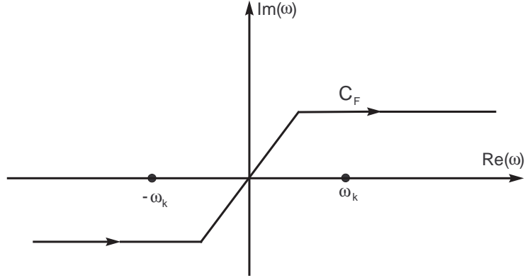
Fig. 7.6 - The integration path C_F .
